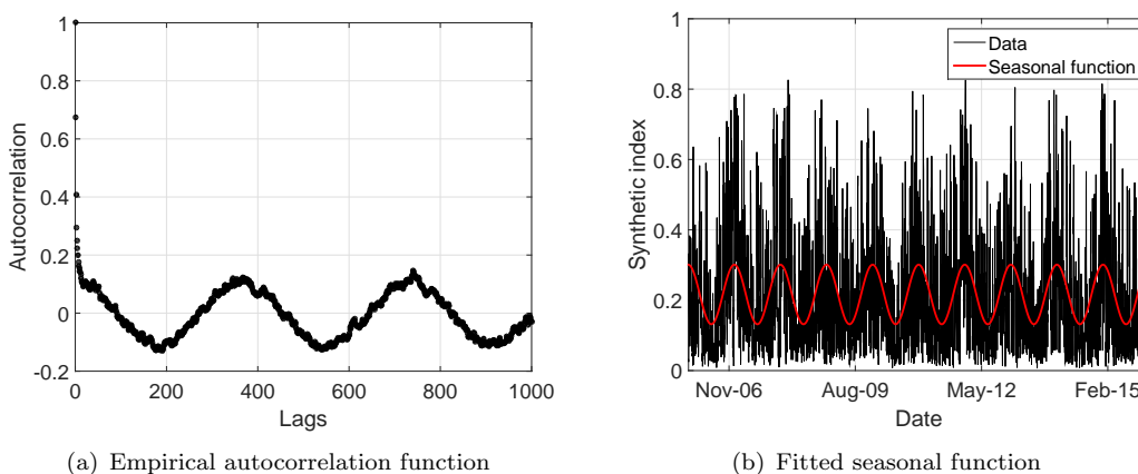
Figure 2. Empirical autocorrelation function of the synthetic wind power production index and fitted seasonal function.
