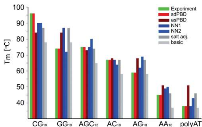
Figure 3. Experimentally determined and calculated melting temperatures of periodic and homogeneous dsDNA sequences. The calculated melting temperatures [ T_m ( ^{\circ}\text{C} ), on the vertical axis] are identified as follows: experimentally determined, green bar; sequence-dependent PBD (sdPBD), red; average stacking PBD (asPBD), brown; NN thermodynamic model (NN1, http://www.promega.com/biomath/calc11.htm ) (16), dark blue; NN thermodynamic model (NN2, http://www.basic.northwestern.edu/biotools/oligocalc.html ) (14,31), light blue; salt adjusted model calculated with a regression ( http://www.promega.com/biomath/calc11.htm ) (32), dark grey; basic regression model ( http://www.promega.com/biomath/calc11.htm ) (33), light grey. The identity of the sequences is shown below the bars.
