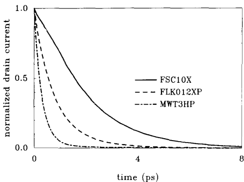
Fig. 2. Drain current responses to a gate voltage pulse for the GaAs MESFETs in Table I. The responses have been normalized to their peak value in order to make the comparison between different devices easier.
