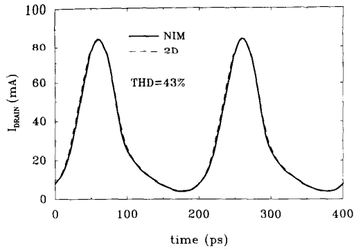
Fig. 3. Plots of the time-varying drain current in a GaAs MESFET amplifier with sinusoidal input at 5 GHz ( P_{IN} = 10 dBm, V_{GS0} = -2 V, V_{DS0} = 4 V). The large-signal performance predicted by the NIM (—) is in good agreement with 2D physics-based numerical device simulation (---). The Total Harmonic Distortion is 43%.
