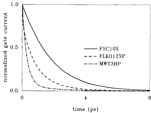
Fig. 1. Gate current responses to a gate voltage pulse for the GaAs MESFETs in Table I. The responses have been normalized to their peak value in order to make the comparison between different devices easier.
