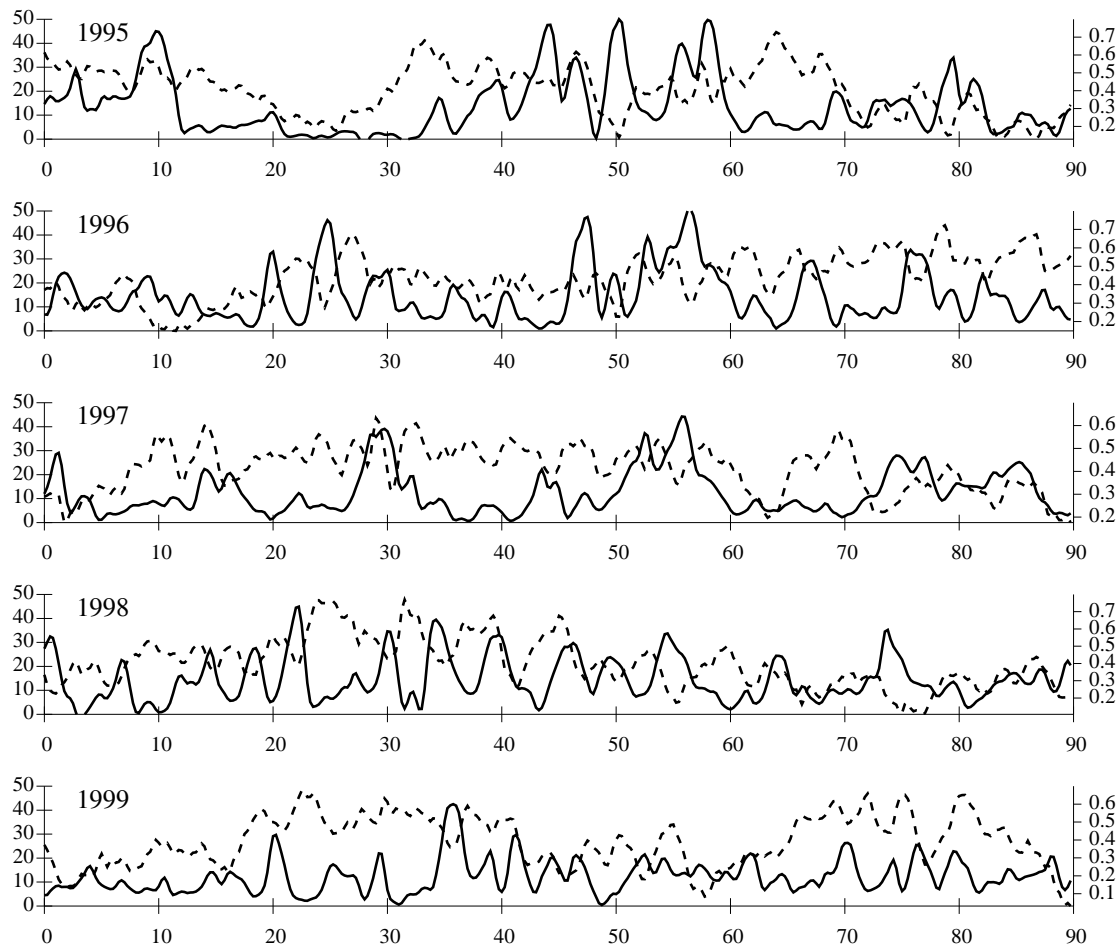
Figure 4. Timeseries of heat flux (solid lines, left axes, units \text{K m s}^{-1} ) and baroclinicity (dashed lines, right axes, units \text{day}^{-1} ) for the DJF winter. Time is in days since 1 December of the indicated year. The heat flux and the baroclinicity are evaluated at the upstream side of the N. Atlantic storm track, as indicated in Fig. 3.
