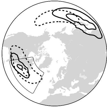
Figure 3. Polar stereographic view of the baroclinicity (solid contours, displaying values of 0.5 and 0.6 day -1 ) and heat flux (dashed contours, displaying values of 10 and 20 K m s -1 ) averaged over the 1957–2002 DJF winters. The sector used for spatial averaging is outlined by the thin solid line.
