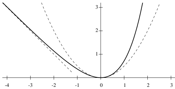
Figure 1. Potential V(y) for nonlinear oscillator in Eq. 8, scaled with 2F , as a function of the transformed heat flux y . The dashed lines correspond to the two asymptotic forms for small y , V(y)/2F \approx y^2/2 , and for negative y , V(y)/2F \approx -y - 1 .
