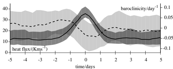
Figure 5. Composite of heat flux and baroclinicity for the winters of 1957–2001, centred around the maxima of the heat flux. The solid line is the median value of the heat flux and the dashed line is the median value of the baroclinicity. The shading corresponds to the interquartile range of each quantity. The anomalous (excess) baroclinicity has been plotted; the mean offset in the baroclinicity is 0.46 \text{ day}^{-1} .
