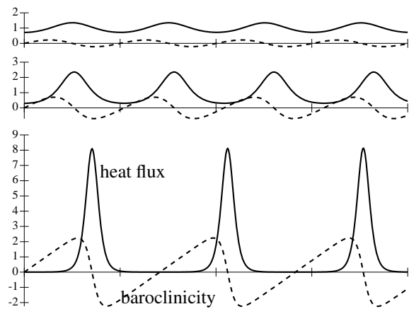
Figure 2. Timeseries of heat flux f (solid lines), rescaled with F , and excess baroclinicity s - s_0 (dashed lines), rescaled with \sqrt{F} . The time is rescaled with the natural frequency of \sqrt{2F} of the system and each tick mark corresponds to one period of this natural frequency. The three panels correspond to E/2F = 0.1 , E/2F = 1 , and E/2F = 10 .
