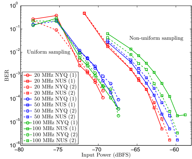
Fig. 16: BER of the decoded GSM signal as a function of input power. Circular markers indicate the performance of the uniform ADC for each of two randomly generated signals (denoted (1) or (2)) at each of three levels of clutter (20, 50 and 100 MHz). Square markers indicate the performance of the NUS on the same signals. The solid and dashed lines correspond to separate trials.
