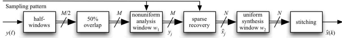
Fig. 12: A block diagram of the practical processing steps.
