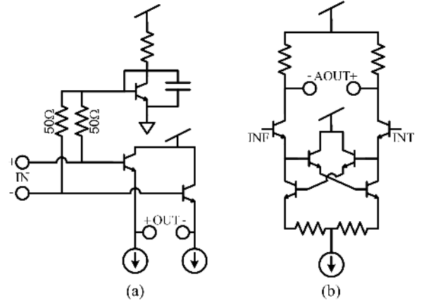
Fig. 5: NUS IC input/output interface circuits. (a) The analog input receiver is a differential 50 Ohm terminated emitter follower. This is a simplified version of the circuit called EF BUF shown in the MSH circuit in Figure 4. (b) The output buffer is a differential quartet design.
