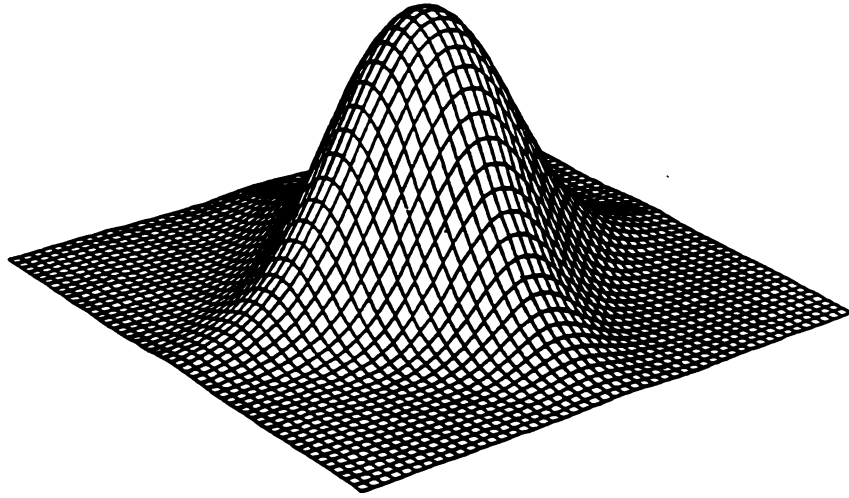
Figure 1. f(x_1, x_2) \propto \exp(-\frac{1}{2}[x_1^2 x_2^2 + x_1^2 + x_2^2])
