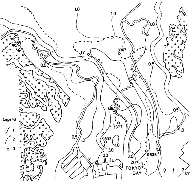
Fig. 4 General outlook of accumulated amount of land subsidence in the Tokyo Lowland since 1929.
