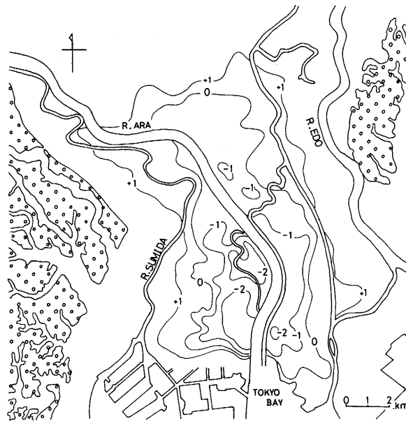
Fig. 5 Ground height (in meters) of the Tokyo Lowland on July 1, 1973.
