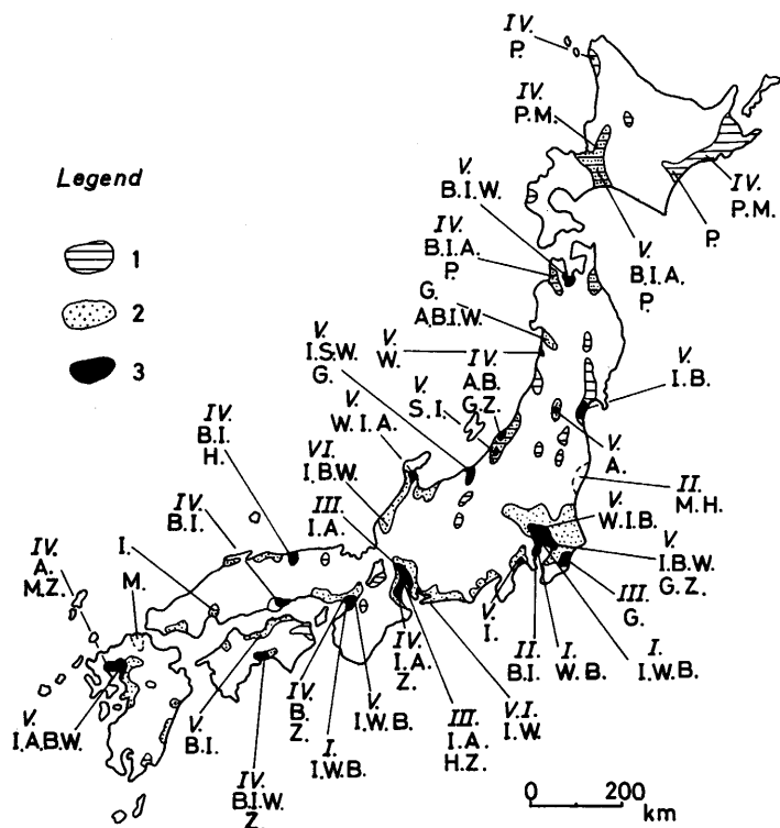
Fig. 1 Distribution and some characteristics of areas in where land subsidence have occurred.
