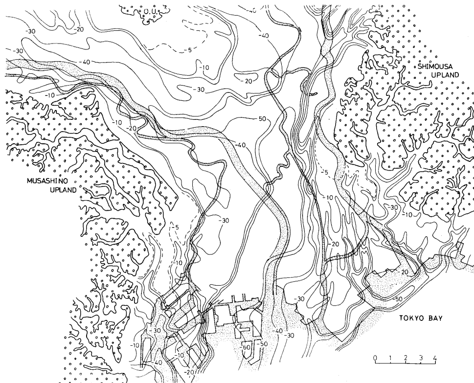
Fig. 2 Basal landform of the recent deposits (heights in meters). O.U. : Omiya Upland.
