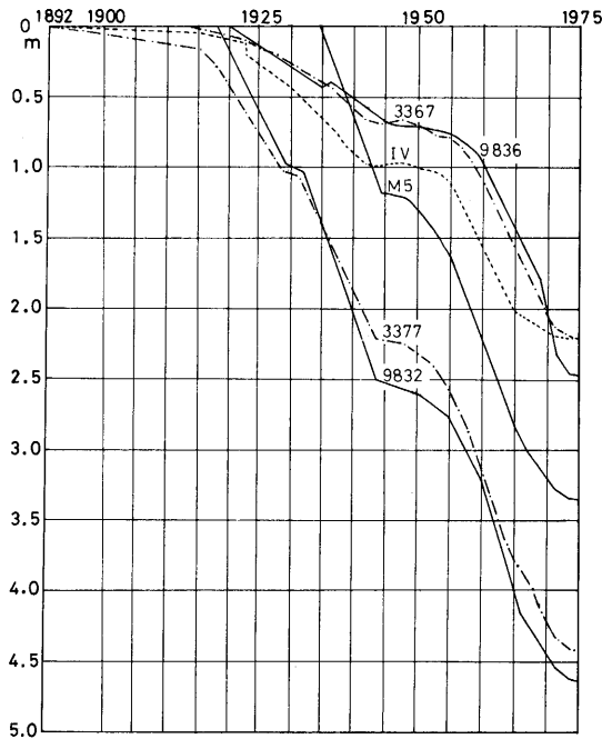
Fig. 3 Integrated land subsidence in the Tokyo Lowland.
