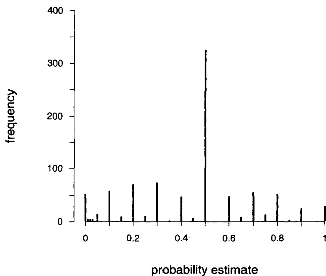
Figure 1. Frequency histogram for all 960 probability judgments collected in the first 3 experiments (4 judgments from each of 240 respondents).
