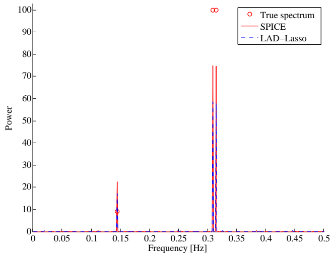
Fig. 1. Spectrum obtained by SPICE and LAD-Lasso.
