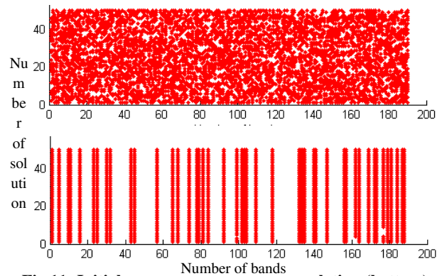
Fig 11: Initial population (top), last population (bottom) after optimizing hyperspectral bands by BHGAPSO for the second test case
