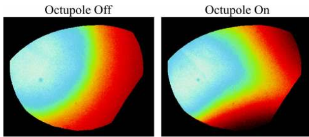
FIG. 3. (Color online) Field lines imaged by passing a circular e^- plasma through the octupole with the octupole off and on. Apertures (Ref. 14) form the image field map. The distortion evident in the right-hand image corresponds to one of the flutes at the end of the magnetic surface shown in Fig. 2.
