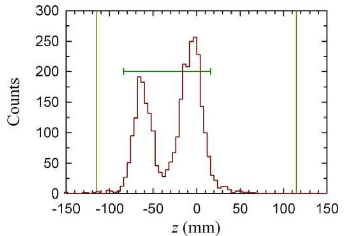
FIG. 5. (Color online) Axial positions where the \bar{p} 's hit the trap wall under the influence of the octupole. The horizontal bar indicates the axial extent and position of the electrostatic well confining the \bar{p} 's. The loss is greatest near the ends of the confining electrostatic well. The positions are determined by a position-sensitive particle detector that monitors the \bar{p} annihilation products; the vertical lines at z = \pm 115 mm indicate the axial extent and position of the detector.
