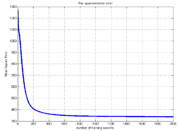
Fig. 19: MSE of FLANN (2-7-3) for \theta_1
