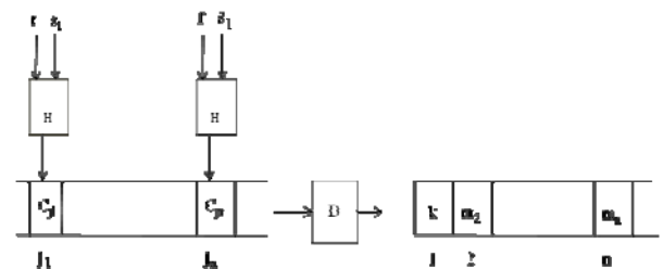
Figure 3. Rekeying-GC's Operations
