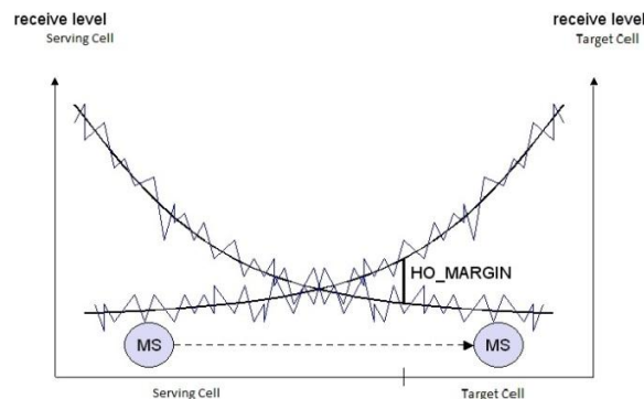
Fig. 4: Conventional Received Signal Strength Based Handover
