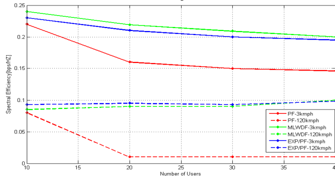
Fig. 9(c) Spectral Efficiency of different schedulers in LTE-SIM [21]
