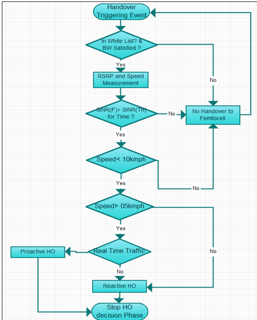
Fig. 8: Proposed Speed Based Handover Model
