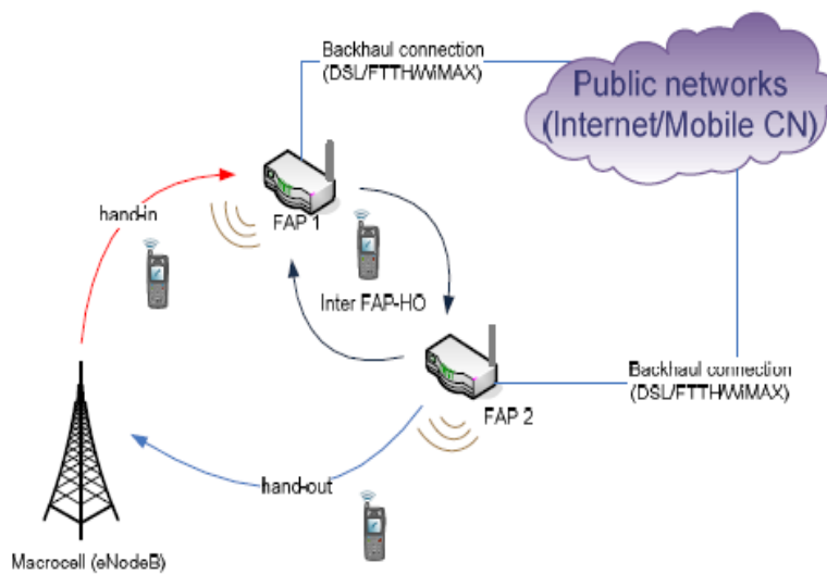
Fig. 2: Handover Scenario in presence of FAP [14]
