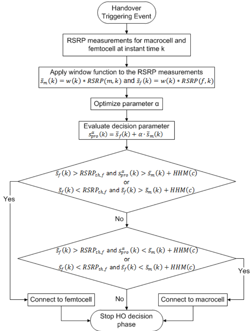
Fig. 5: HO Algorithm based on RSS [10]
