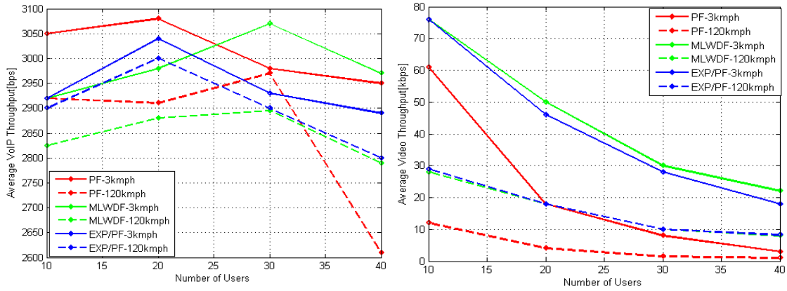
Throughput (VoIP) Throughput (Video) Fig. 9 (a) Average Throughput of VoIP and Video Flow with different schedulers at different speed [21]
