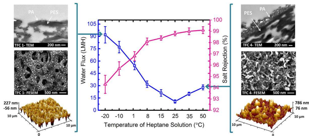
Figure 4. Water flux and salt rejection of the TFC membranes prepared at different temperature in 0.2 wt.% TMC-heptane solution. The surface and cross-sectional images of the membranes synthesized at -20^{\circ}\text{C} and 50^{\circ}\text{C} are presented to justify the permeation properties. Test conditions: feed solutions: pure water and 2000 ppm NaCl solution, pressure: 1.52 Mpa (220 psi), temperature: 25^{\circ}\text{C} , pH: 6.5–7.
