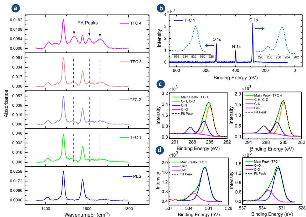
Figure 3. (a) FTIR spectra (PES support and TFC1-4), (b) XPS survey spectrum (TFC 1) along with high resolution C (1s) and O (1s) spectra, (c) convolved high resolution C (1s) and (d) convolved high resolution O (1s) spectra (TFC 1 & TFC4). FTIR shows additional peaks associated with the PA to the PES support. The survey spectrum indicates the presence of O, N and C elements and the absence of S on the surface of the membranes indicating all membranes are integrally skinned. The convolved high resolution C (1s) and O (1s) peaks provide information about the PA chemical bonds that helps to quantify C=O/C–N ratio. The high resolution C (1s) and O (1s) spectra of TFC 2 and TFC 3 membranes are presented in Supplementary Information.
