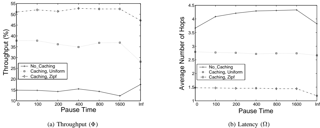
Fig. 5. Throughput ( \Phi ) and latency ( \Omega ) as a function of pause time.
