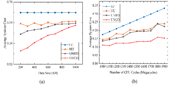
Fig. 4. The impact of data size and CPU cycles on average system cost
