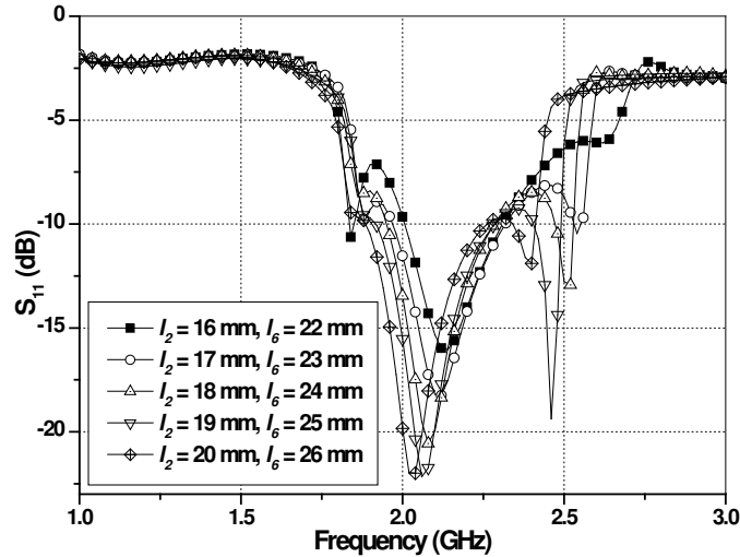
Fig. 5. S_{11} against frequency with different l_2 and l_6 .
