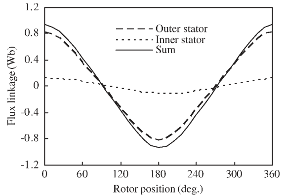
Fig. 7. Flux linkages.
