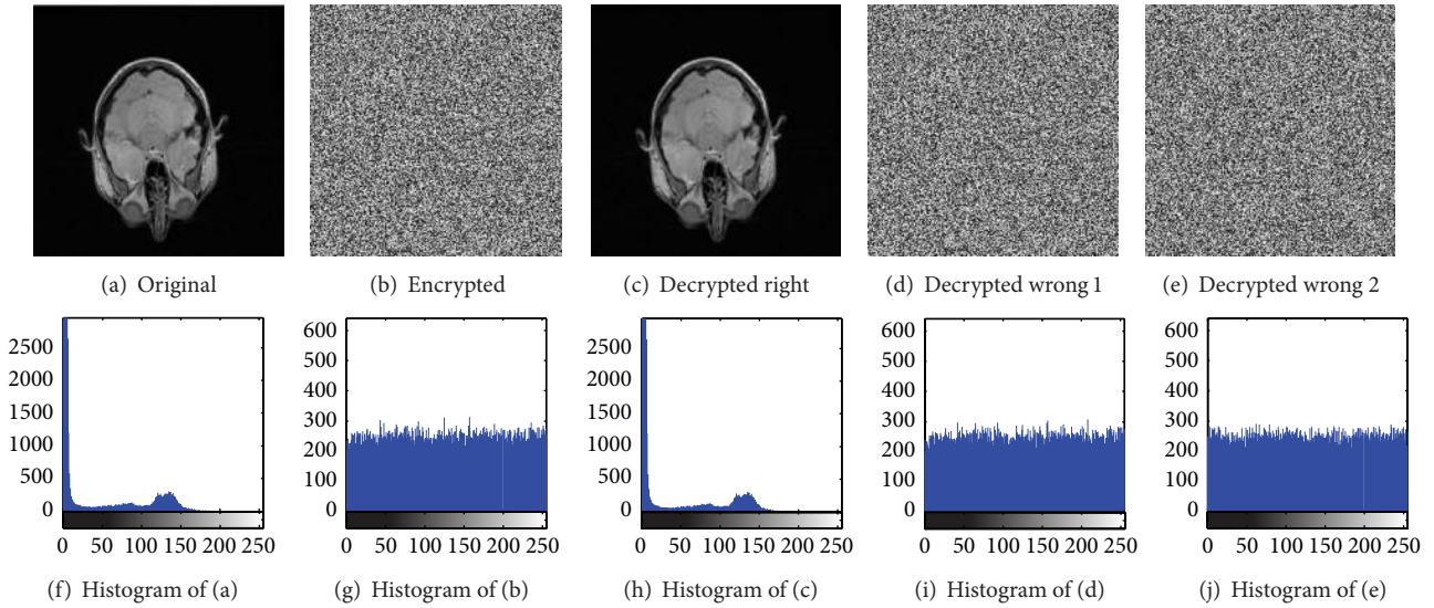
FIGURE 8: Encryption and decryption of medical image with size 256 \times 256 .
