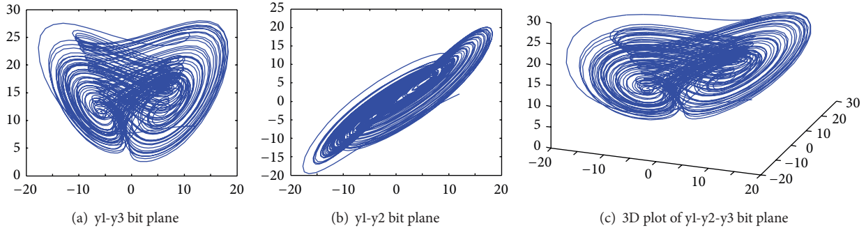
FIGURE 3: Hyperchaotic attractors of system (2).
