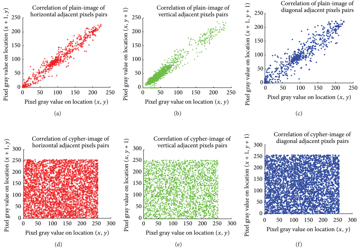
FIGURE 10: Correlations of two adjacent pixels in the plain-image and in the cipher-image of im11.
