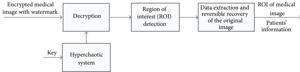
FIGURE 2: Block diagram of decryption and information extraction.
