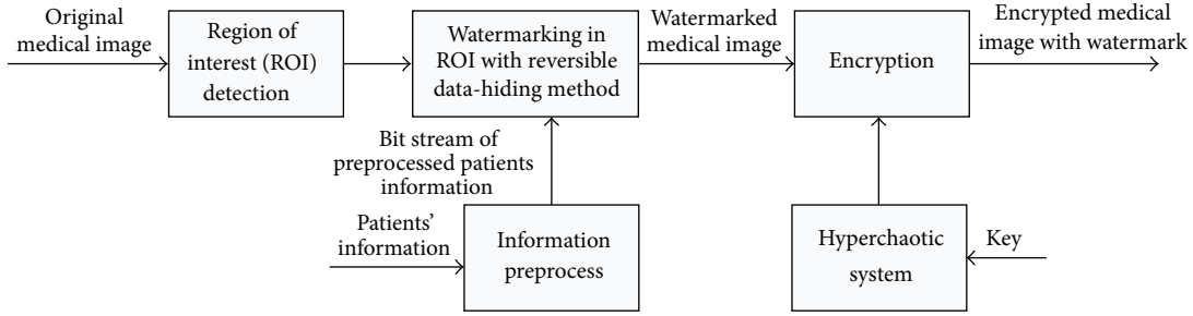
FIGURE 1: Block diagram of information embedding and encryption.
