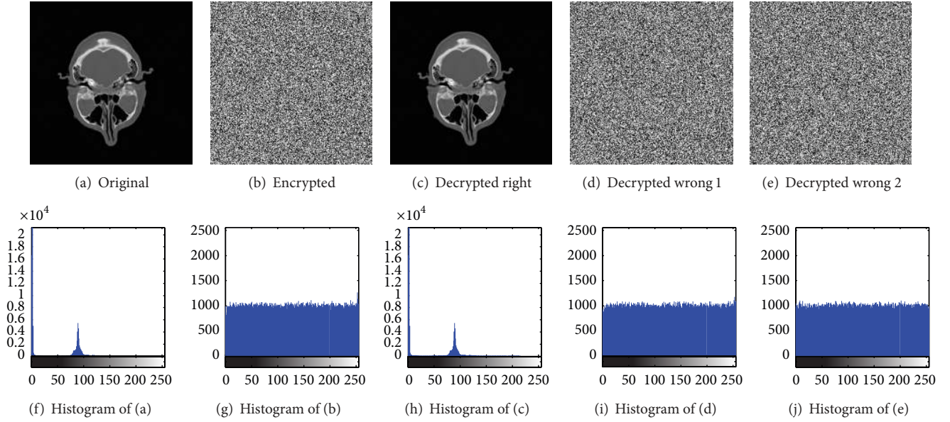
FIGURE 7: Encryption and decryption of medical image with size 512 \times 512 .
