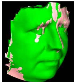
(c) Quality=0.02
