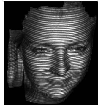
(b) Decompressed 3D image by JPEG2000, Quality=21%, 3D RMSE=4.02
