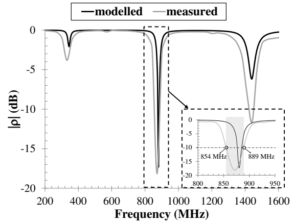
Fig. 10. Measured and modelled reflection coefficient in the UHF band (normalized to 12\ \Omega ). 0.5\text{-}\lambda , 1.5\text{-}\lambda and 2.5\text{-}\lambda resonances can be clearly recognized.
