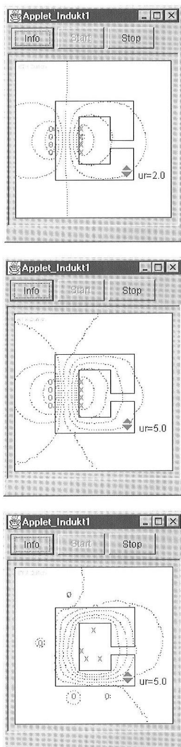
Fig. 4. Magnetic field of an inductor. By changing the permeability (denoted as “ ur ” in the applet) of the magnetic core one can see how the magnetic flux distribution is influenced by magnetic material.
