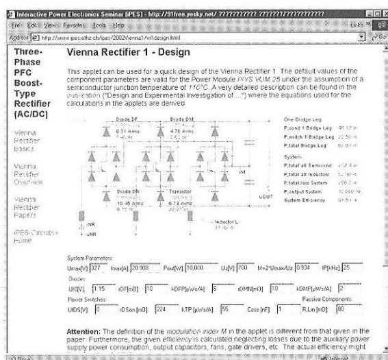
Fig. 2. Principle of operation of the Vienna Rectifier I (left hand side) and (b) Java applet facilitating the dimensioning of the Vienna Rectifier I power circuit (right hand side).
