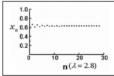
Figure 1. Response of Logistic Map for \lambda=2.8
