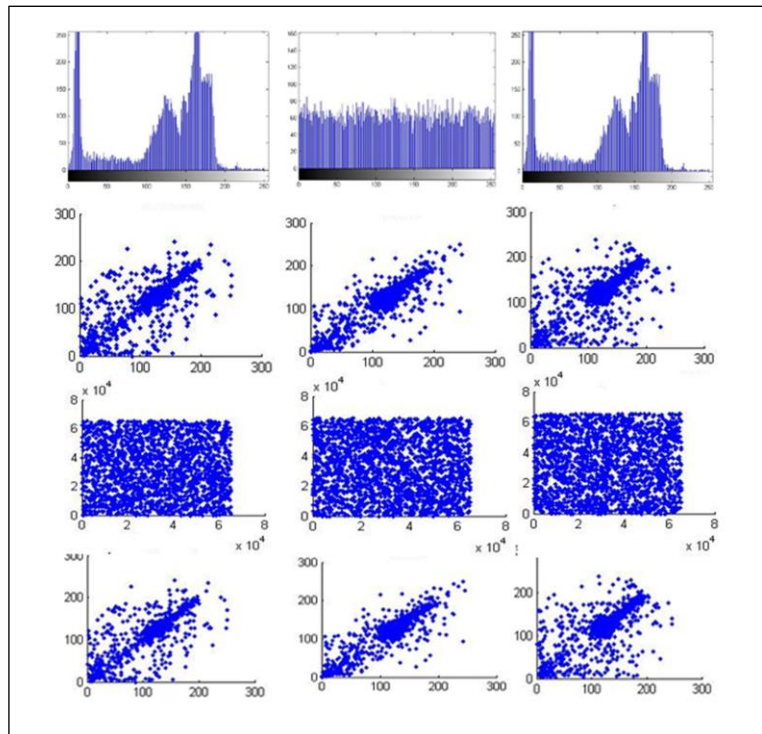
Figure 5. In the First Row Histogram Representation of the Cameraman standard Image (from left to right: Original, Encrypted and Decrypted), From Second Row-, Top to Bottom : Correlation Coefficients of Original, Encrypted and Decrypted, Left to Right: Correlation Coefficients in Horizontal, Vertical and Diagonal Directions
