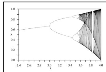
Figure 3. Bifurcation Diagram of Logistic Map
