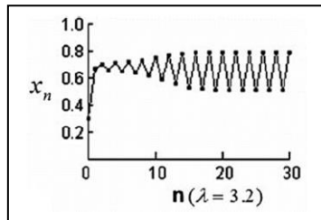
Figure 2. Response of Logistic Map for \lambda=3.2
