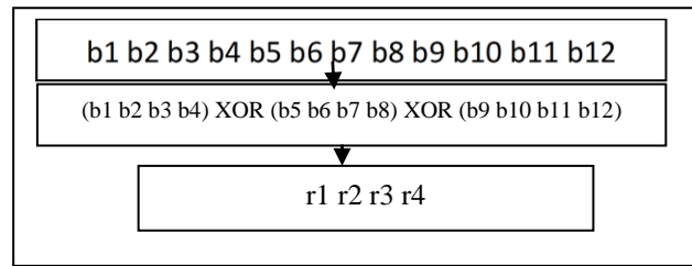
Figure 4. 4 Bit Key Generation from 12 Bit Sequence
