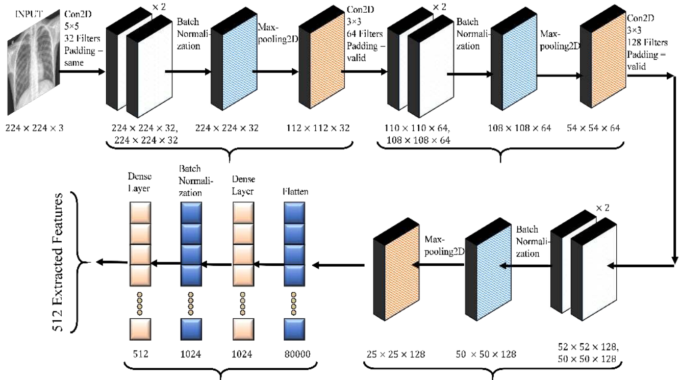
Figure 3. Proposed CNN model for features extraction.
