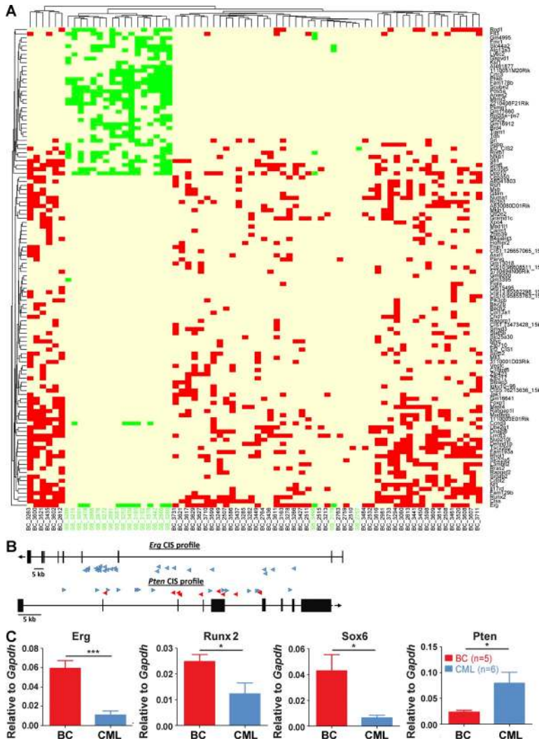
Figure 7. Transposon leads to transcriptional de-regulation and a distinct mutational signature in the BC cohort. (A) Unsupervised analysis of BC ( n = 52 ) and SB ( n = 20 ) insertion profiles by Euclidean distance, based on insertion number and identity. Each column represents an individual case with BC insertions in red and SB in green. (B) Insertions in the Erg gene were all found in the sense strand (blue arrows), strong indication of activating events. Conversely, insertions on the Pten gene were found in both strands (anti-sense strand in red arrows), suggesting inactivation of this gene. (C) Gene expression levels of selected CIS genes were investigated by qRT-PCR (BC, n = 5 ; CML, n = 6 ). Data are representative of at least three independent experiments. Student's t test was used. Data are mean \pm SEM. *, P < 0.05 ; ***, P < 0.0001 .
