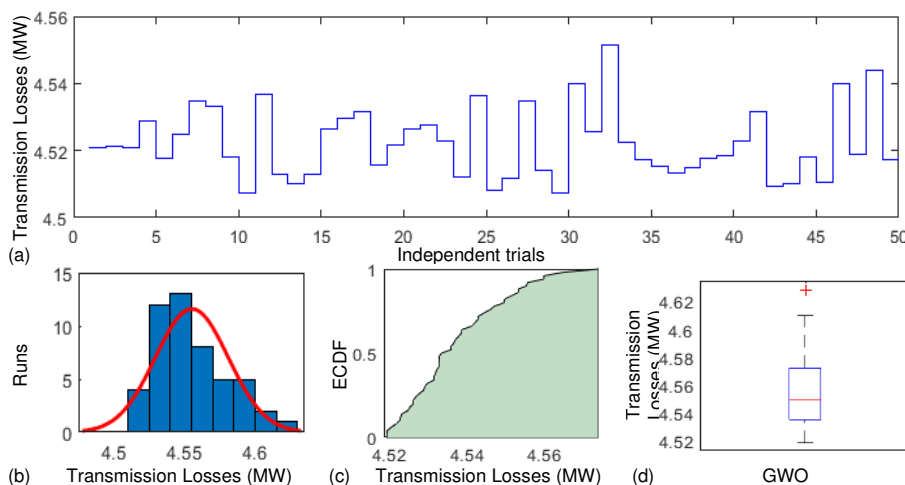
FIGURE 13. Statistical Analysis of GWO for Transmission Losses Minimization on IEEE30 Bus for 19 Variables – CASE B
