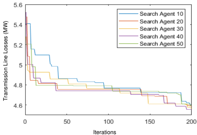
FIGURE 8. GWO Convergence Curve on Different Search Agents for Fitness Objective ( F_1 ), IEEE30 (19 Variables) – CASE B
