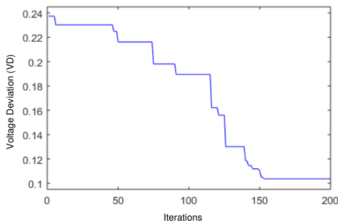
FIGURE 5. Convergence Curve of GWO for Fitness Objective ( F_2 ), IEEE30 (13 Variables) – CASE A
