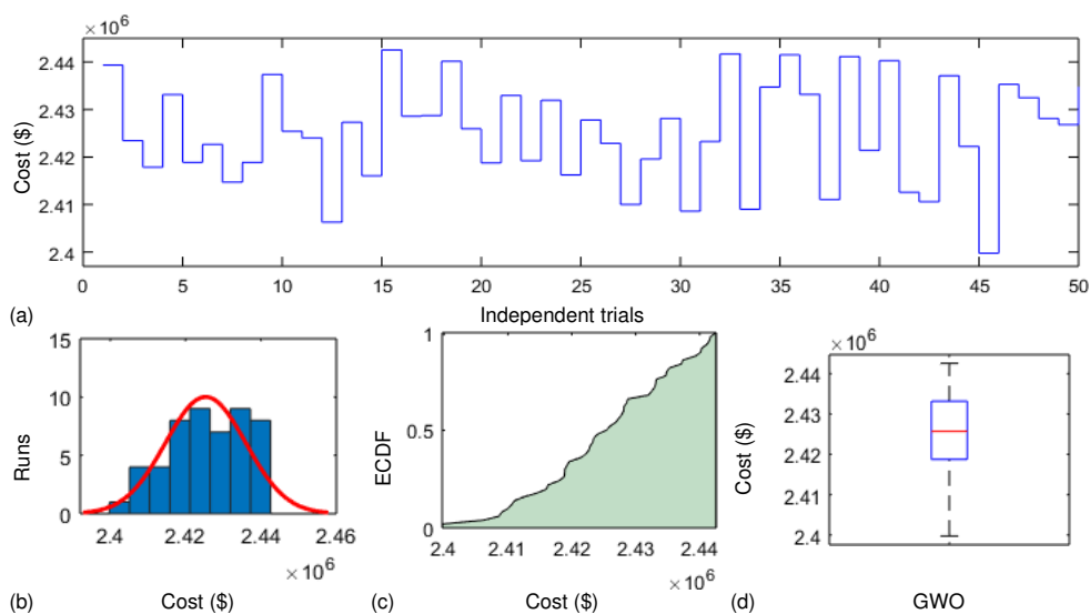
FIGURE 19. Statistical Analysis of GWO for Cost Minimization on IEEE30 Bus for 19 Variables – CASE B
