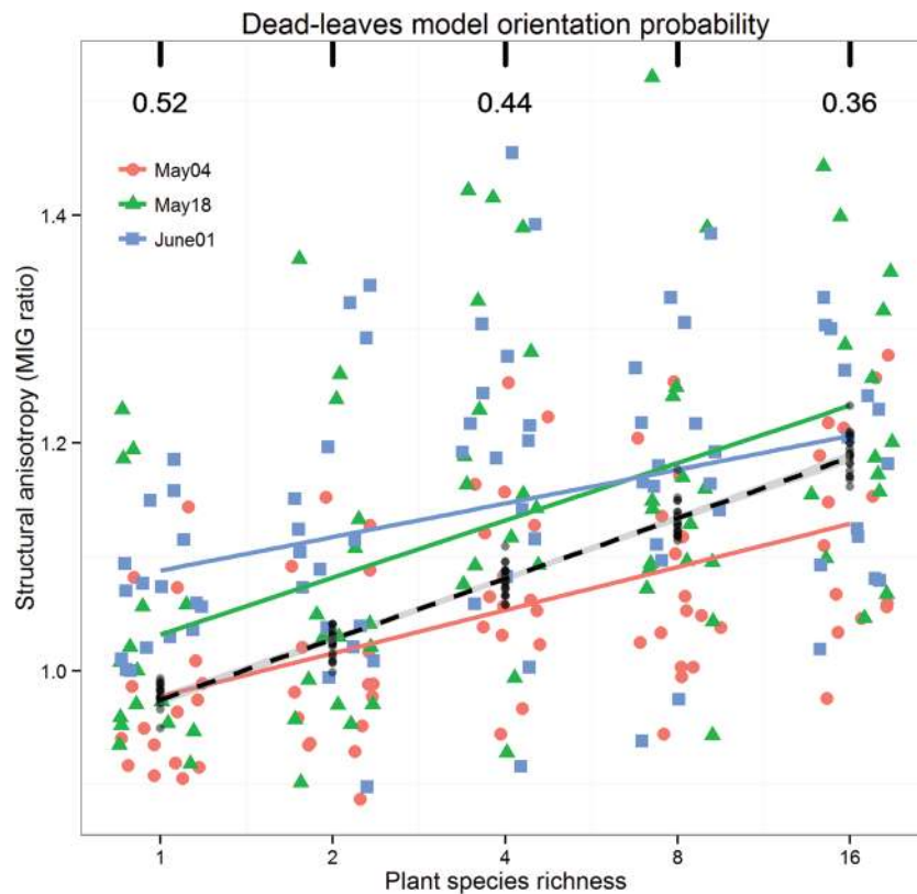
Figure 3: effect of plant species richness on anisotropy ( MIG_{\text{horizontal}}/MIG_{\text{vertical}} ), a measure of structural heterogeneity calculated from the gray-tone images of 78 grassland communities photographed on three different occasions (May 04, May 18 and June 01). Plant species richness is expressed on a logarithmic scale, while anisotropy values at each richness level appear slightly jittered. Are superimposed the results of a dead-leaves geometric model (dashed black line), in which the orientation probability is a parameter determining the probability that the major axis of an ellipsoid object in the image falls along the horizontal direction. A total of 20 gray-tone images were simulated at each of five orientation probability values: 0.52, 0.48, 0.44, 0.40 and 0.36.
