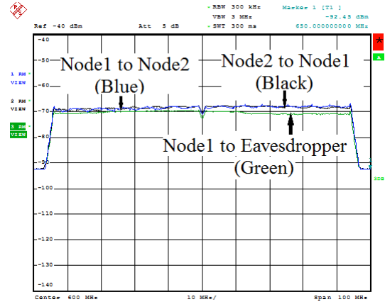
Fig. 13. Screenshot of measured channel responses between legitimate nodes and the eavesdropper.
