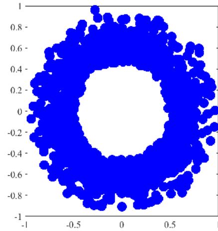
Fig. 16. First 1000 symbols of the received encrypted 8PSK signal before decryption and equalization.
