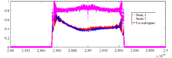
Fig. 6. Normalised convolved channel and hardware frequency responses.
