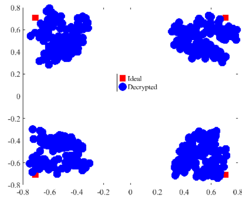
Fig. 19. Recovered QPSK constellation of OFDM sub-carriers received over the 28.9 GHz wireless link.
