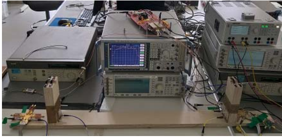
Fig. 11. Test bench used for validation. Node 1 is on the left. Node 2 and Node 3 are on the right. Node 3 is connected to a vector signal analyzer.
