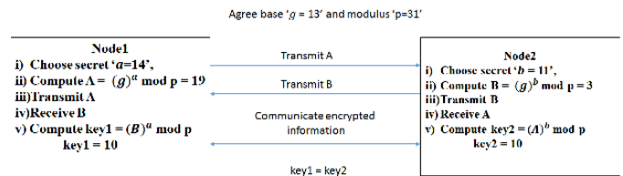
Fig. 2. Example of diffie hellmann Key exchange.
