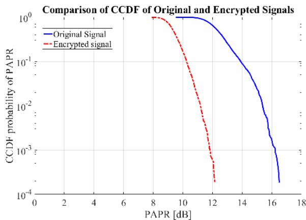
Fig. 20. CCDF of PAPR of original and encrypted 2048 point OFDM modulated signals with 1664 active sub-carriers.
