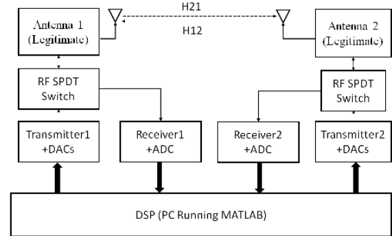
Fig. 14. Apparatus used for symmetric key generation.
