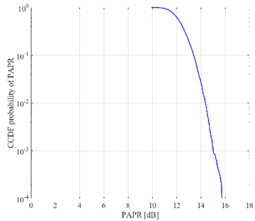
Fig. 1. CCDF plot of a 2048 point OFDM signal with 1664 QPSK modulated sub-carriers exceeding threshold PAPR values.
