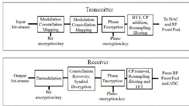
Fig. 9. Proposed PHY encryption and decryption in the transmitter and the receiver of OFDM systems.
