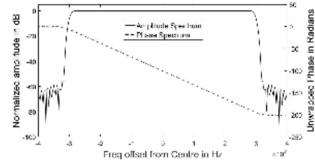
Fig. 8. Frequency response of a hamming windowed filter.
