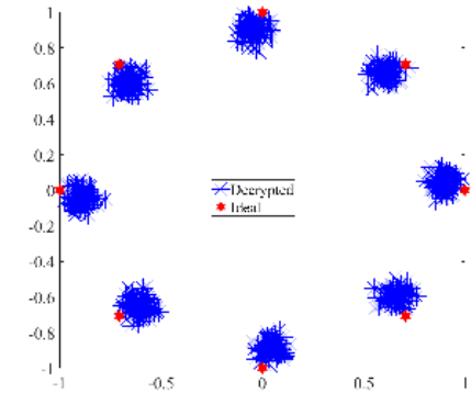
Fig. 17. Recovered 8PSK constellation after decryption filtering and equalization.
