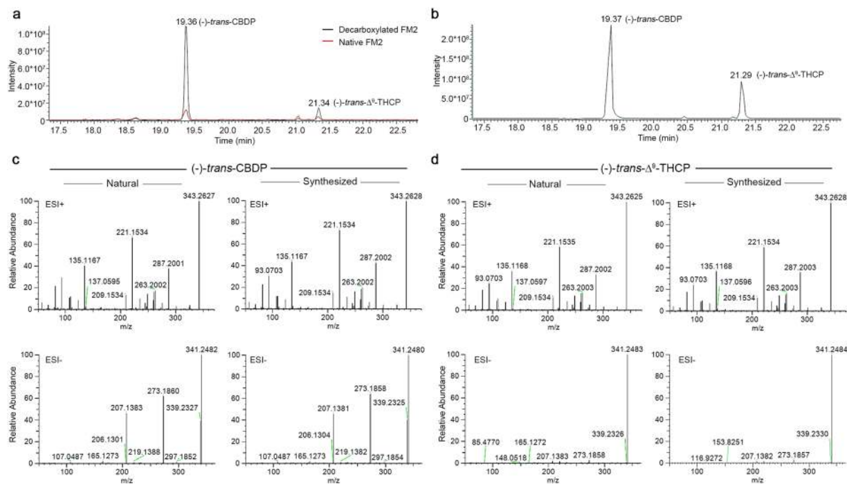
Figure 1. UHPLC-HRMS identification of (-)-trans -CBDP and (-)-trans - \Delta^9 -THCP. Extracted ion chromatograms (EIC) of CBDP and \Delta^9 -THCP from a standard mixture at 25 and 10 ng/mL respectively (a) and from the native (red plot) and decarboxylated (black plot) FM2 (b). (c,d) Comparison of the high-resolution fragmentation spectra of synthetic and natural CBDP and \Delta^9 -THCP in both positive (ESI+) and negative (ESI-) mode.
