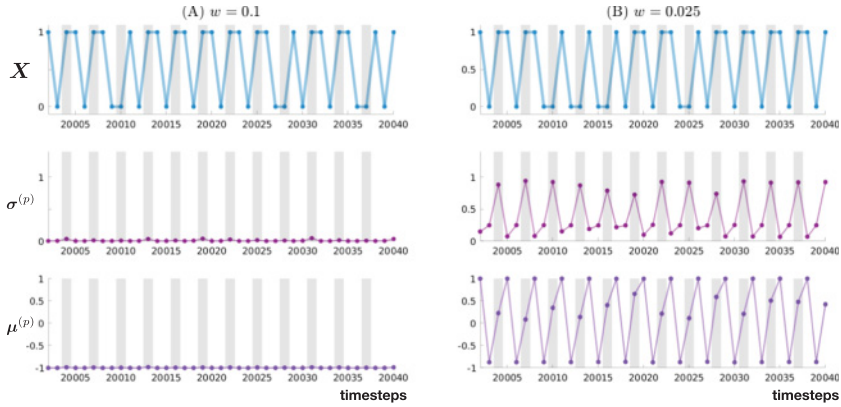
Figure 5: The generated output, the mean \mu^{(p)} , and the standard deviation \sigma^{(p)} from time steps 20,002 to 20,040 of two PV-RNNs trained with the meta-prior w set to 0.1 (A) and 0.025 (B). Gray bars show the time steps corresponding to uncertain states.
