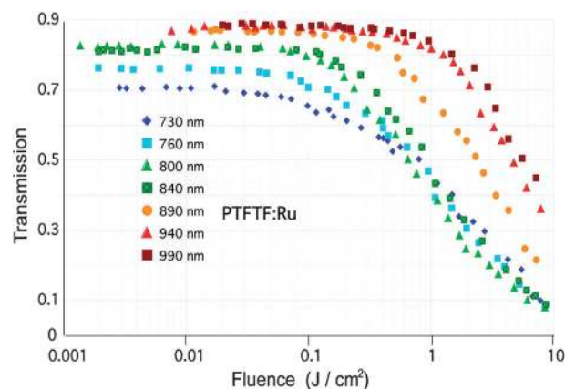
Fig. 9 Nonlinear transmission curves in chloroform between 730 and 990 nm of PTFTF:Ru complex at 50 \text{ g l}^{-1} .
