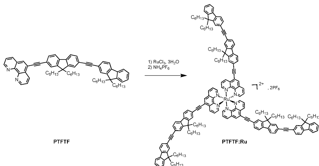
Fig. 1 Molecular structures of the PTFTF ligand and the PTFTF:Ru complex.
