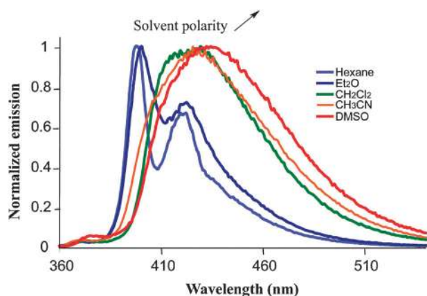
Fig. 5 Emission spectra of the PTFTF ligand in a series of solvents.
