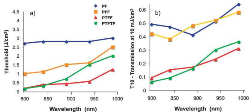
Fig. 10 Th (a) and T_{10} (b) variations between 800 and 990 nm for PTFTF:Ru , PTFF:Ru , PFF:Ru , and PF:Ru complexes at 50 \text{ g L}^{-1} (figures represent experimental points and lines are given for clarity of the lecture).
