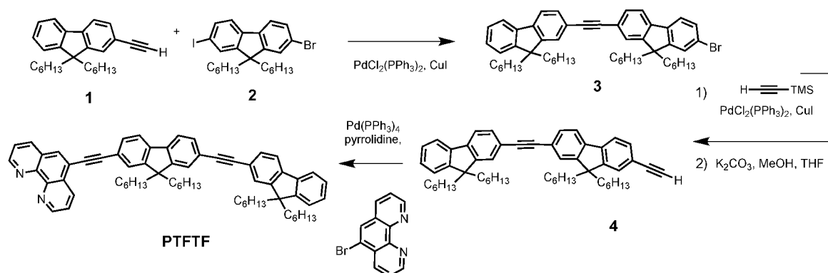
Fig. 2 Synthesis of the PTFTF ligand.
