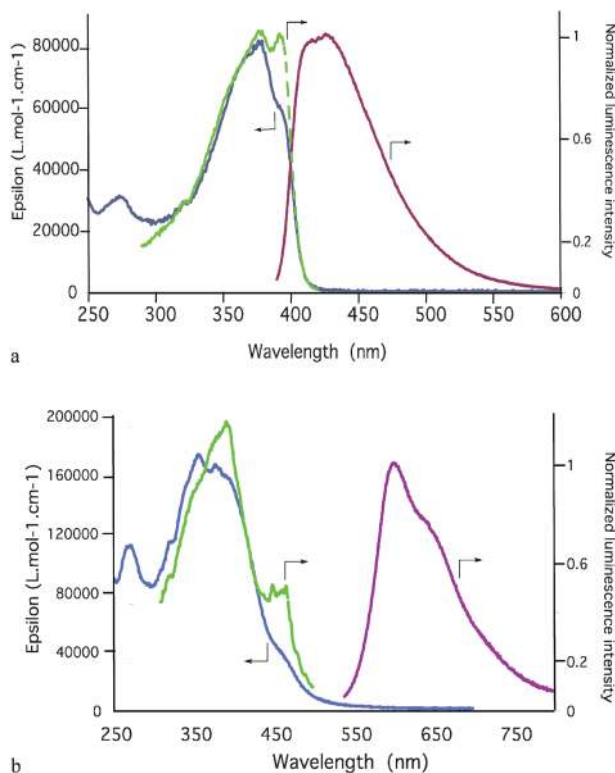
Fig. 4 Absorption (in chloroform), excitation (dotted line, in dichloromethane) and normalised emission spectra (in dichloromethane) of PTFTF (a) and the related PTFTF:Ru complex (b).
