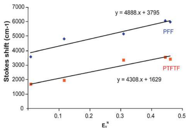
Fig. 6 (a) Plot of Stokes shift ( \Delta\nu_{\text{ST}} ) against Dimroth-Reichardt E_{\text{T}}^{\text{N}} parameter (see Table 2) and correlation according to eqn (2) of the Stokes shift and the Lippert-Mataga polarity parameter for compounds PFF and PTFTF in the five solvents listed in Table 1 ( R^2 = 0.93 for both compounds).
