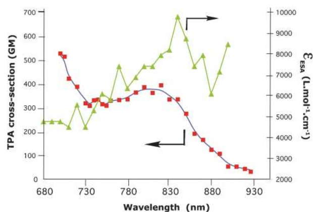
Fig. 8 TPA and ESA spectra of PTFTF:Ru in chloroform (the experimental uncertainty is \pm 15\% ); figure represents ESA coefficients experimental points; lines are given for clarity of the lecture.
