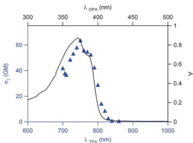
Fig. 7 Two-photon excitation spectrum of PTFTF measured in acetonitrile (the experimental uncertainty is \pm 15\% ). For comparison, linear excitation spectrum of this ligand was also reported.
