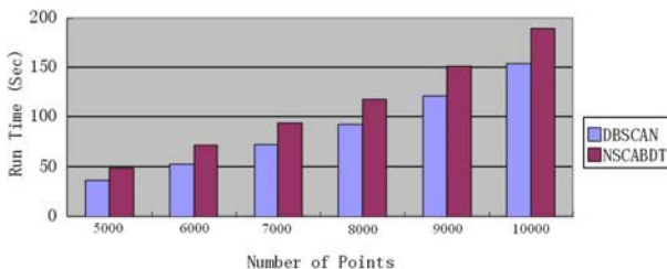
Figure 8. Efficiency: SCABDT VS DBSCAN
