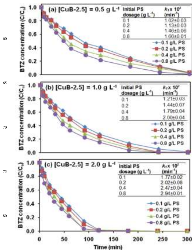
Fig. 7: BTZ removal at various initial PS dosage and (a) 0.5 \text{ g L}^{-1} , (b) 1.0 \text{ g L}^{-1} and (c) 2.0 \text{ g L}^{-1} of CuB-2.5. Conditions: [\text{BTZ}]_0 = 2.5 \text{ mg L}^{-1} and [\text{pH}]_0 = 7 .
