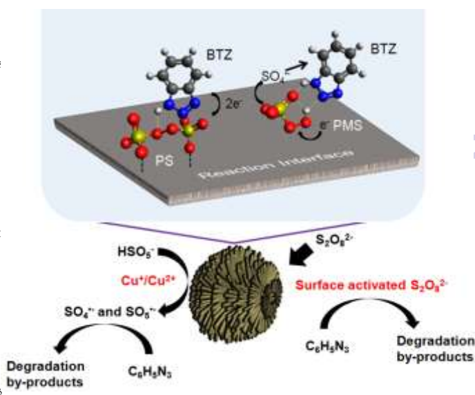
Fig. 6: Schematic illustration of the mechanisms of PS and PMS activations by CuB-2.5 for BTZ degradation.
