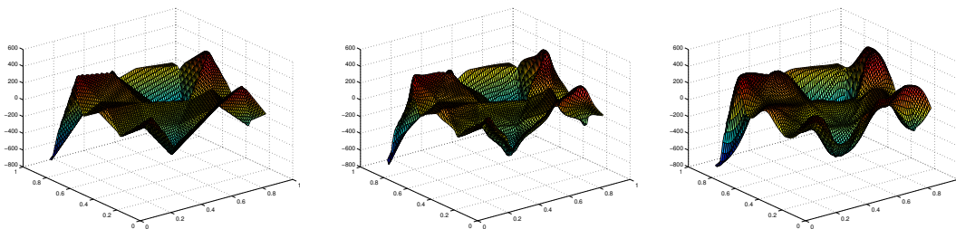
Figure 2: Left: \omega(\lambda) = \lambda . Center: \omega(\lambda) = \log(1 + 1000\lambda^3) . Right: \omega(\lambda) = \lambda^3 e^{-3\lambda} .
