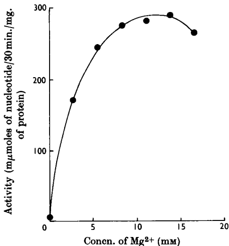
Fig. 3. Effect of the concentration of Mg 2+ on the breakdown of DNA by streptomycin-treated extracts of iron-limited Myco. smegmatis. Incubation mixtures were as described in the text, except that the Mg 2+ concentration was varied. Soluble acid-labile deoxyribose was determined and correction was made for pyrimidine-bound material.
