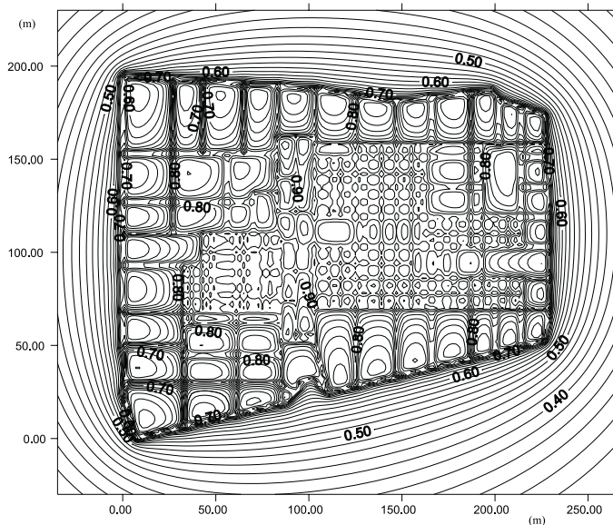
Fig. 4. Santiago II grounding system: Potential distribution ( \times 10 kV) on ground surface obtained with a two layer soil model.
