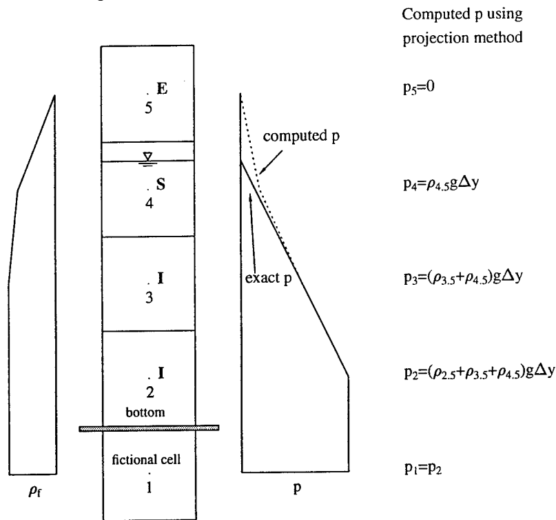
Figure 5: An example of PPE computations for one-dimensional problem
