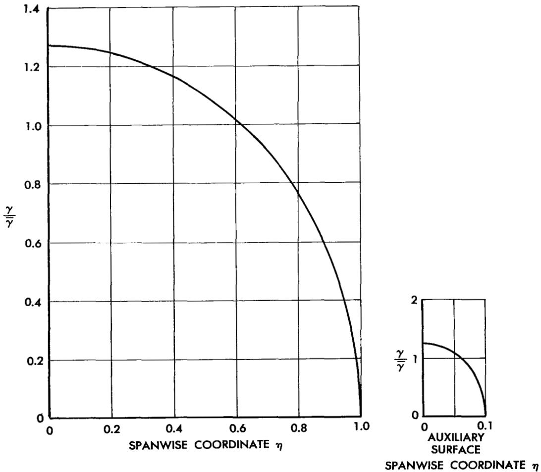
Figure 16. Loading for Minimum Induced Drag on a Biplane
