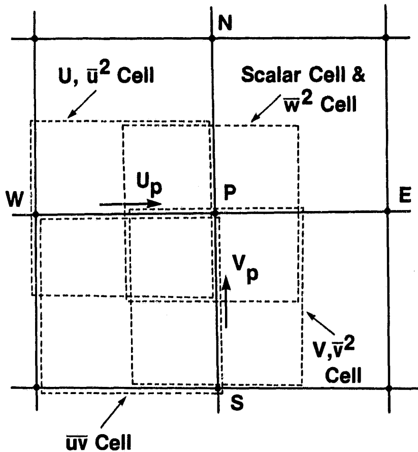
Fig. 1 The grid, storage locations and control volumes. • , grid point, -----, control surface.
