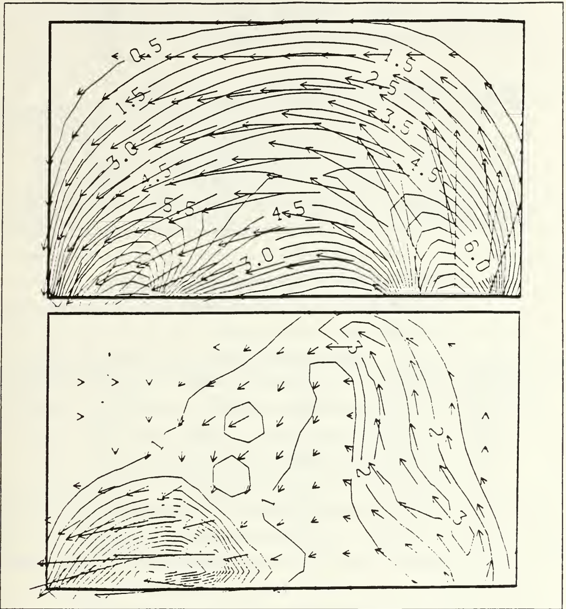
Figure 10. Reference state forced at the south side of the bay: The upper and lower figures respectively represent the upper and lower layer velocity fields for the reference state forced at the southern side of the offshore section. Isotachs are drawn at 0.5 cm/sec and 1 mm/sec intervals for the upper and lower figures respectively. North is to the left in each figure and each figure represents a 32.7 by 19.0 km domain.
