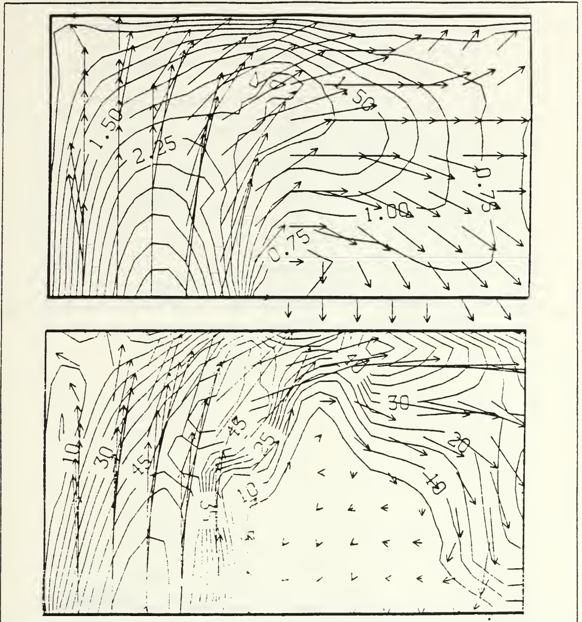
Figure 15. Experiment No.5 (N. inflow, topography, and 5/5 shear): The upper and lower figures respectively represent the upper and lower layer velocity fields for Experiment No. 5. Isotachs are drawn at 0.25 cm/sec and 5 mm/sec for the upper and lower figures respectively. North is to the left in each figure and each figure represents a 32.7 by 19.0 km domain.
