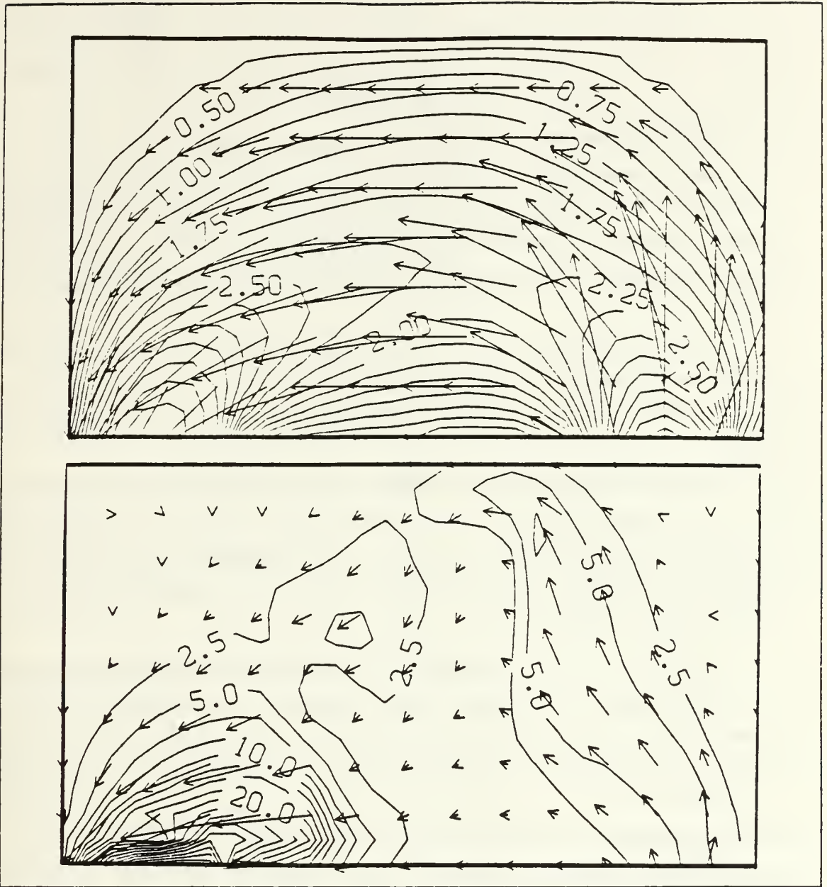
Figure 17. Experiment No.7 (S. inflow, topography, and 5/2 shear): The upper and lower figures respectively represent the upper and lower layer velocity fields for Experiment No. 7. Isotachs are drawn at 0.25 cm/sec and 2.5 mm/sec intervals for the upper and lower figures respectively. North is to the left in each figure and each figure represents a 32.7 by 19.0 km domain.
