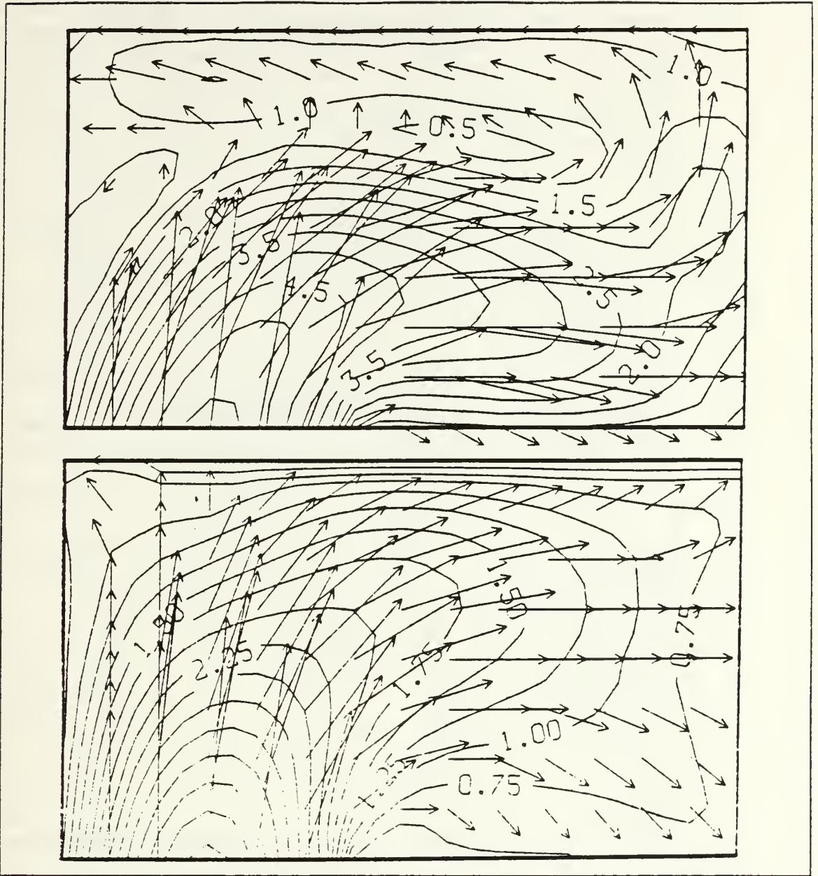
Figure 13. Experiment No.3 (N. inflow, topography, and 10/5 shear): The upper and lower figures respectively represent the upper and lower layer velocity fields for Experiment No. 2. Isotachs are drawn at 0.5 and 0.25 cm/sec intervals for the upper and lower figures respectively. North is to the left in each figure and each figure represents a 32.7 by 19.0 km domain.
