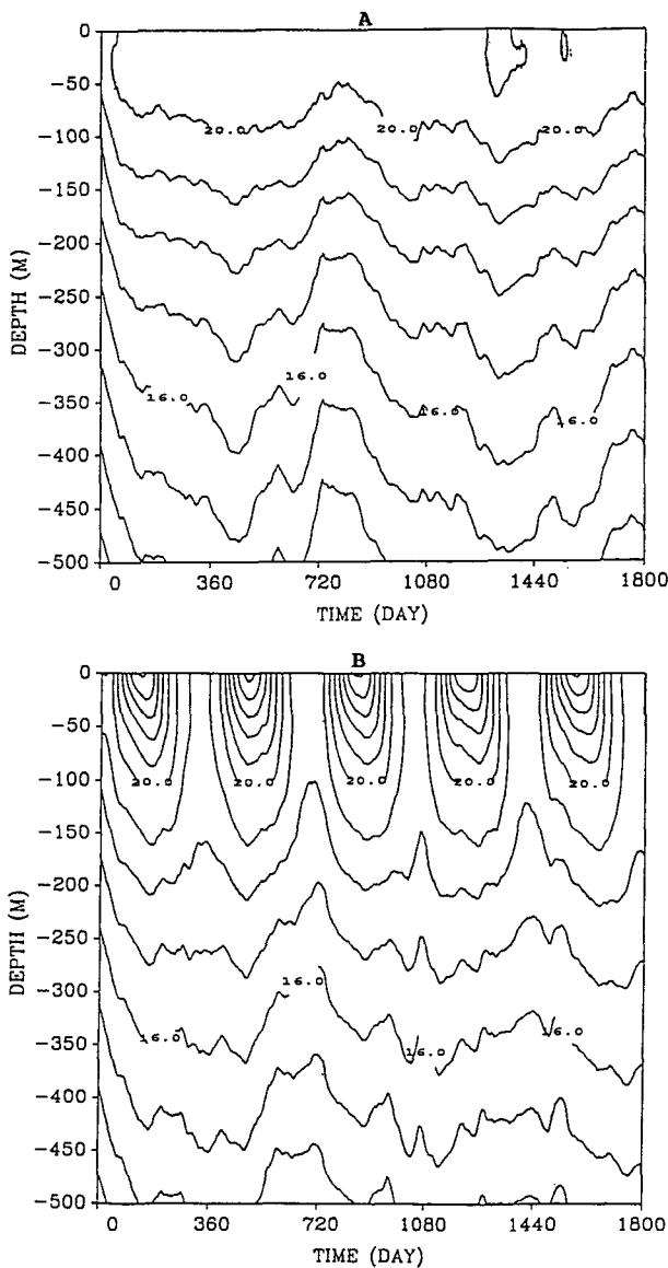
FIG. 11. The temperature structure in the upper 500 m, in experiment 3 (upper panel) and experiment 4 (lower panel). Contour interval is 1°C.
