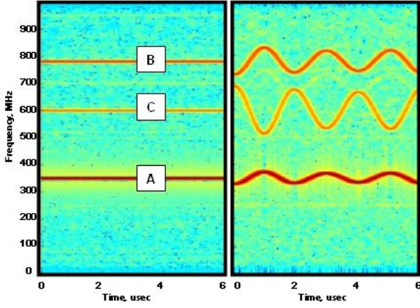
Figure 4: Multi-Signal Lab Test Example
