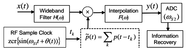
Figure 1: Nyquist Folding A-to-I Receiver Architecture
