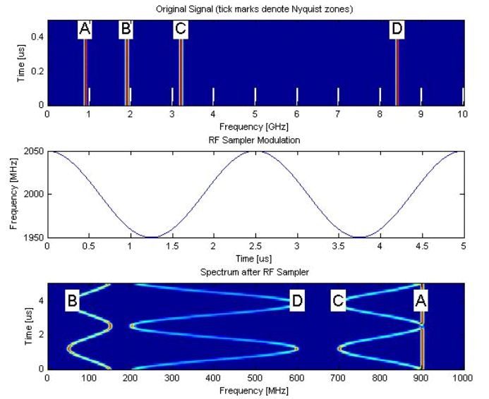
Figure 3: Sinusoid FMCW Sample Clock Signal Example
