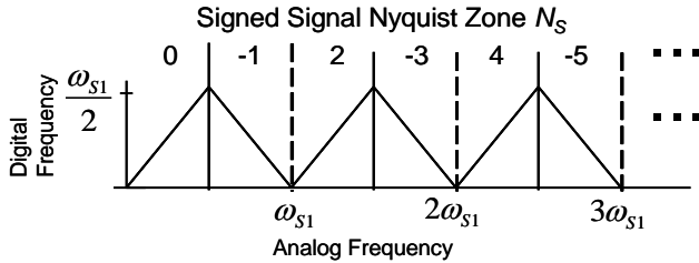
Figure 2: Bandpass Sampled Signal Nyquist Zones
