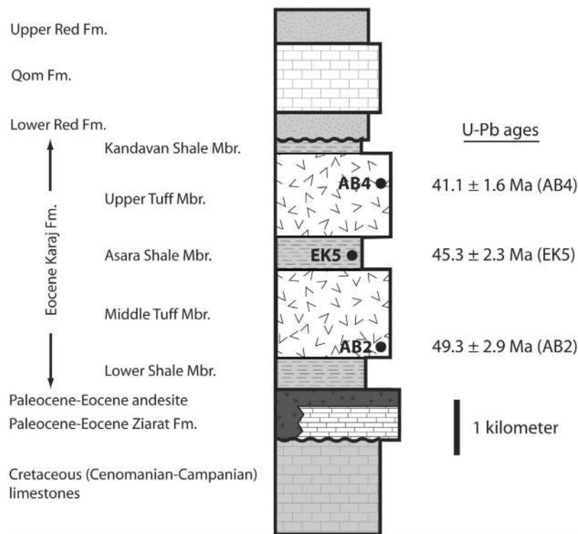
Figure 4. Cretaceous through Miocene stratigraphy of the Chalus Road area summarizing geochronological results (modified from Haghipour et al. [1987]). Thicknesses are approximate. Sample numbers in parentheses. Sample EK5 is a tuff within the Asara Shale Member.
