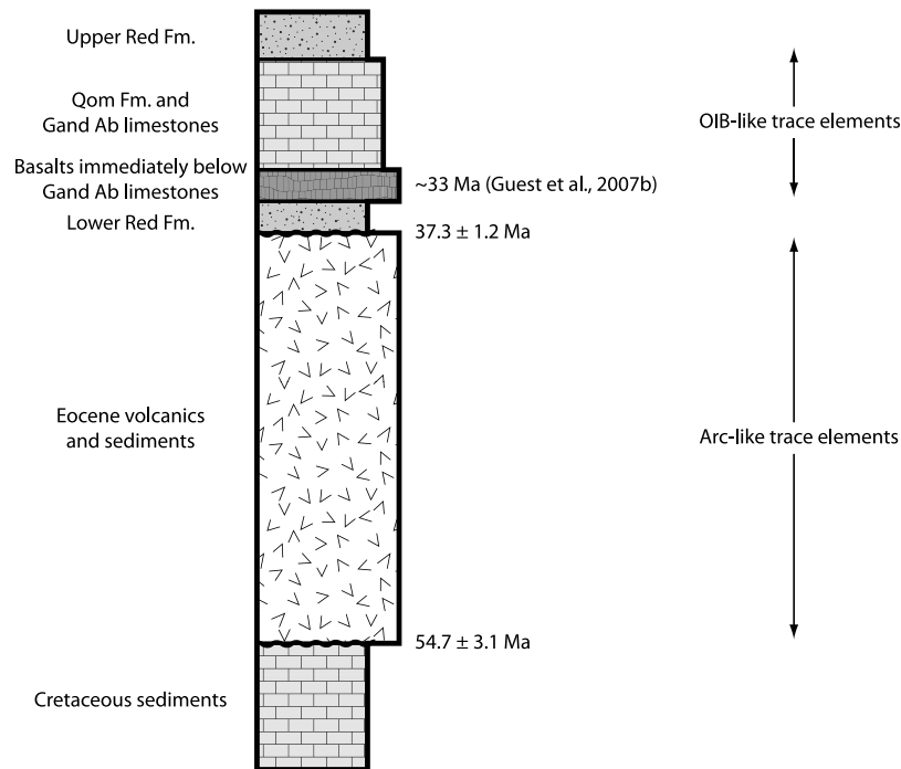
Figure 7. Generalized Tertiary stratigraphy of Iran showing key radiometric age constraints.
