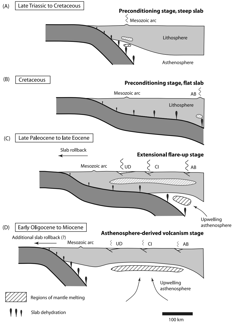
Figure 8. Summary of the development of the Iranian Eocene flare-up and subsequent asthenosphere-derived Oligocene magmatism. (a) Late Triassic to Cretaceous slow subduction generated limited magmatism within the Sanandaj-Sirjan zone. (b) Cretaceous flat slab subduction shifted the locus of magmatism to the Alborz Mountains. During this and the earlier stage, lithospheric mantle beneath the overriding plate was preconditioned by dehydration of subducted Neotethyan oceanic crust. (c) Late Paleocene to late Eocene slab rollback extended and thinned the overriding plate, leading to decompression melting of preconditioned lithospheric mantle and the formation of metamorphic core complexes and elongate rift basins. Magmatic contributions from upwelling asthenosphere were overwhelmed during this stage by the contribution from the fertilized lithospheric mantle. (d) Extension continued during the late Oligocene to Miocene during deposition of the Qom Formation. The flare-up ended when the supply of fertile, preconditioned lithospheric mantle was exhausted, at which time asthenosphere-derived, OIB-type volcanism became dominant. Miocene Arabia-Eurasia collision ended the extensional period and inverted the rift basins. Abbreviations: UD, Urumieh-Dokhtar magmatic belt; AB, Alborz Mountains; CI, central Iranian Eocene volcanics between Urumieh-Dokhtar and the Alborz Mountains.
