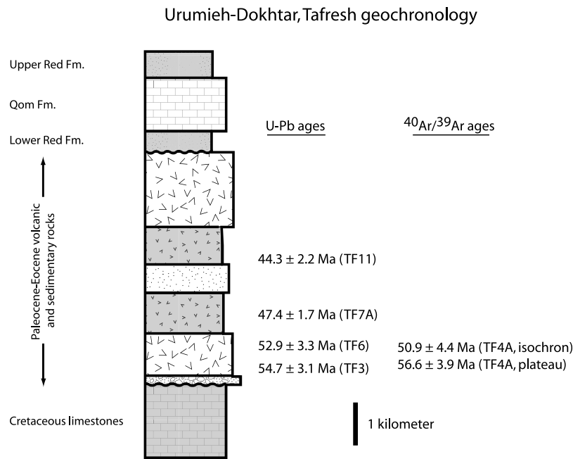
Figure 3. Composite stratigraphy of Cretaceous through Miocene volcanic and sedimentary rocks in the Tafresh area (modified from Emami [1991]) showing general stratigraphic position of geochronology samples. Thicknesses are approximate. Sample numbers in parentheses.
