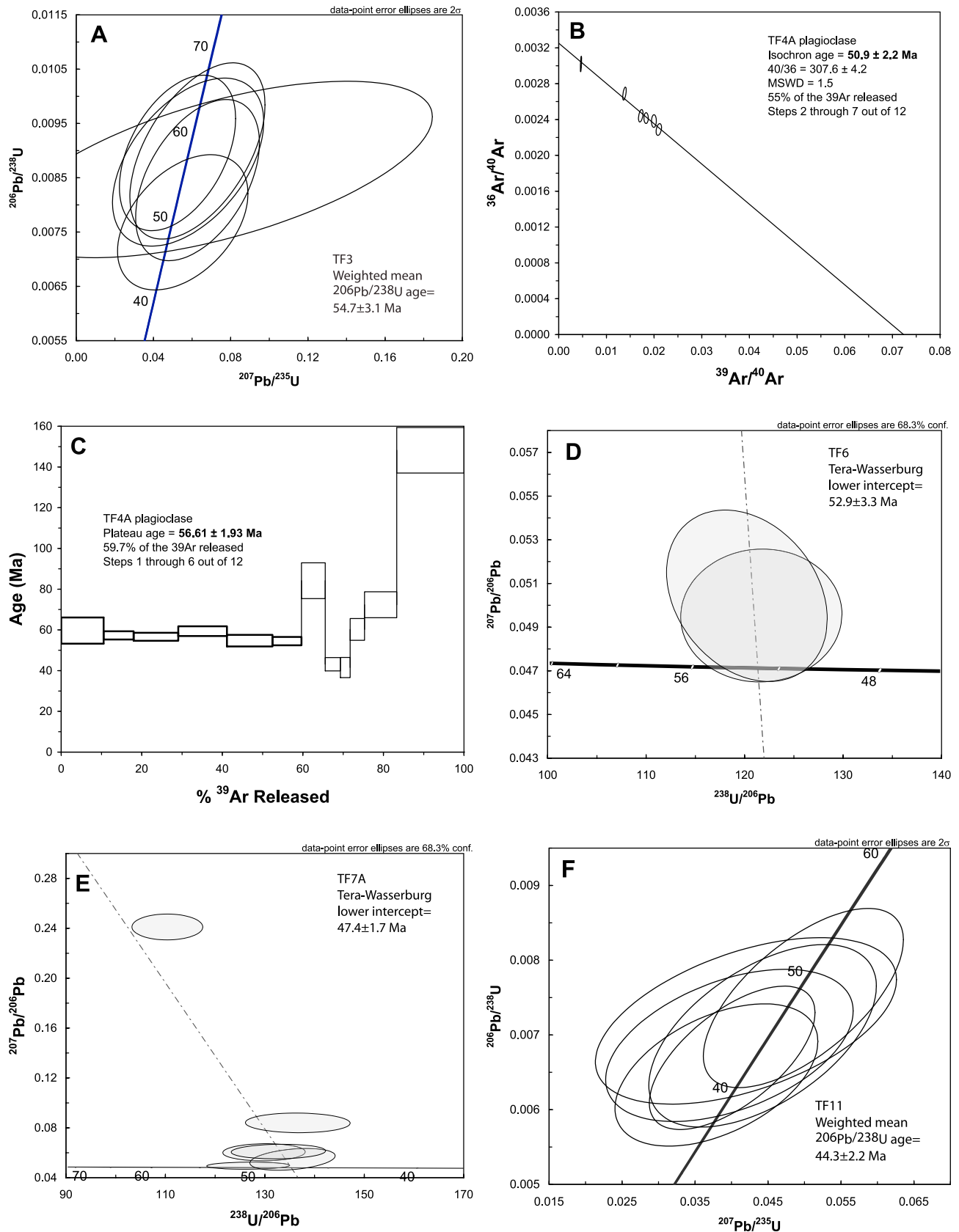
Figure 2. (a-k) U-Pb and ^{40}\text{Ar}/^{39}\text{Ar} geochronology data for volcanic rocks from the Alborz Mountains and the Urumieh-Dokhtar belt.
