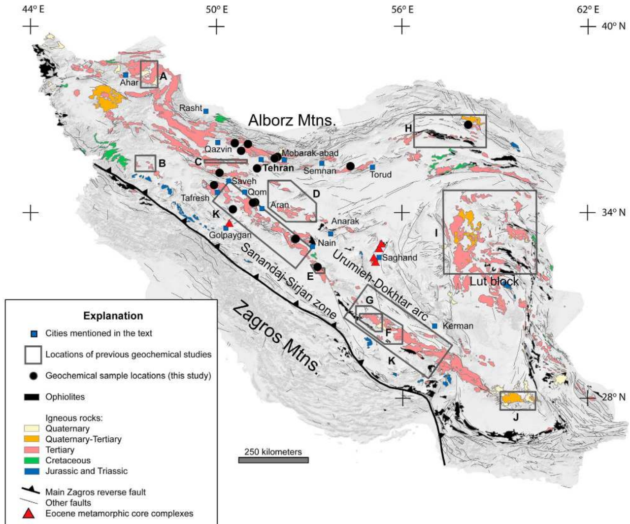
Figure 1. Map of Iran highlighting Cenozoic and Mesozoic igneous rocks (modified from Haghipour and Aghanabati [1985] and Pollastro et al. [1999]). Eocene metamorphic core complexes from Moritz et al. [2006] and Verdel et al. [2007]. Previous geochemical studies: A, Alberti et al. [1979]; B, Boccaletti et al. [1976]; C, Ghorbani [2006]; D, Amidi et al. [1984]; E, Amidi and Michel [1985]; F, Förster et al. [1972]; G, Hassanzadeh [1993]; H, Spies et al. [1984]; I, Jung et al. [1984]; J, Dupuy and Dostal [1978]; K, Omrani et al. [2008].
