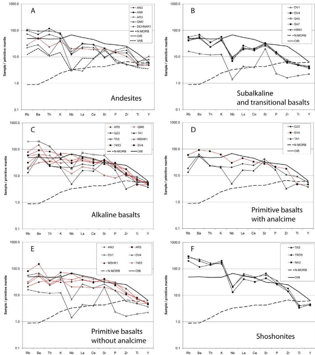
Figure 6. Primitive mantle normalized trace element diagrams. Eocene samples shown in black, and Oligocene shown in red. (a) Andesites, (b) subalkaline and transitional basalts, (c) alkaline basalts, (d) primitive basalts with analcime, (e) primitive basalts without analcime, (f) shoshonites. Primitive mantle, N-MORB, and OIB values from Sun and McDonough [1989]. Volcanic arc basalt (VAB) values from Hickey et al. [1986].
