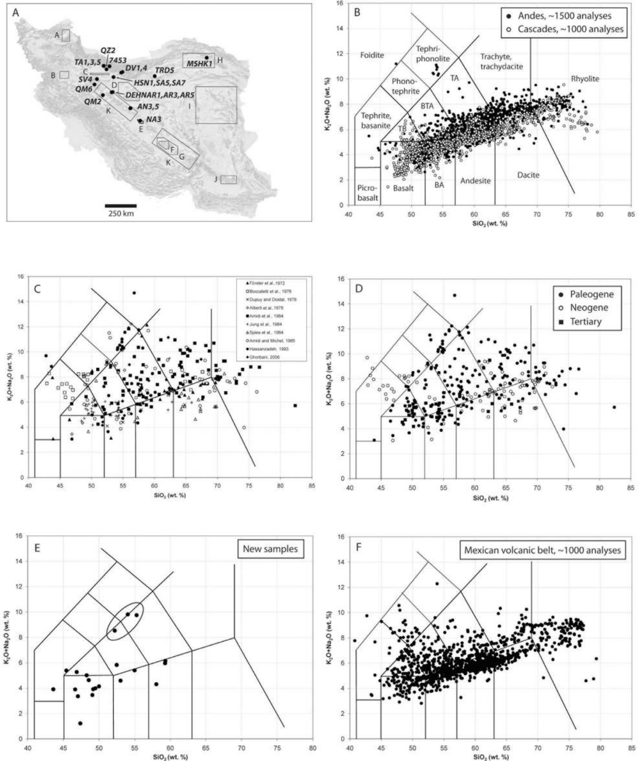
Figure 5. Total alkali-silica diagrams. (a) Sample locations and previous geochemical studies A-K as in Figure 1. (b) Data from ~1500 Andean samples and ~1000 Cascades samples, compiled from the GEOROC database. Nomenclature is also shown. Abbreviations: BA, basaltic andesite; BTA, basaltic trachyandesite; TA, trachyandesite; TB, trachybasalt. (c) Data from ~300 Iranian Tertiary samples, compiled from the sources shown in Figure 5a. (d) Same data as Figure 5c coded by age. (e) Twenty-one new Iranian Tertiary samples; oval drawn around shoshonitic samples. (f) Approximately 1100 samples from the Mexican volcanic belt, compiled from the GEOROC database.
