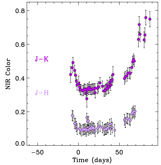
Figure 12. Evolution of the optical and NIR colors. While SN 2009ip clearly evolves toward redder optical colors starting from t_{\text{pk}} - 3 days, no strong evolution is apparent in the NIR colors in the same time interval.
