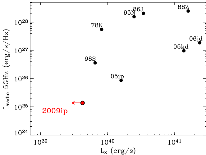
Figure 26. Radio luminosity at peak vs. X-ray luminosity at the radio peak for a sample of Type II In SNe (black dots). SN 2009ip is shown in red. Data have been collected from the literature (Pooley et al. 2002; Smith et al. 2007; Stritzinger et al. 2012; Chandra et al. 2009, 2012a; Pooley et al. 2007; Chandra & Soderberg 2007; Zampieri et al. 2005; Houck et al. 1998; Chevalier 1987; van Dyk et al. 1993; Fabian & Terlevich 1996 and references therein).
