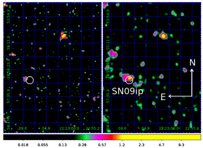
Figure 9. Left panel: Swift -XRT image of the field of SN 2009ip collecting data before and after the optical peak ( -32 \text{ days} < t - t_{pk} < -2 \text{ days} and +29 \text{ days} < t - t_{pk} < +83 \text{ days} ), for a total exposure time of 110 ks. Right panel: the same field imaged around the optical peak ( -2 \text{ days} < t - t_{pk} < +13 \text{ days} ), for a total exposure time of 86 ks. In both panels a white circle marks a 10'' region around SN 2009ip. X-rays are detected at a position consistent with SN 2009ip around the optical peak (right panel) with a significance of 6.1\sigma . (A color version of this figure is available in the online journal.)
