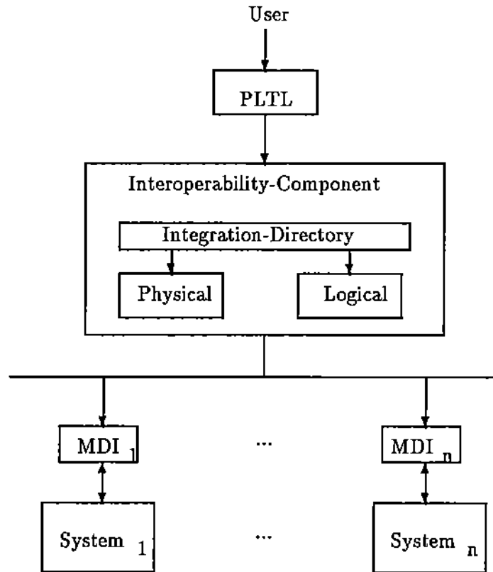
Figure 1: An architecture for multidatabase systems
