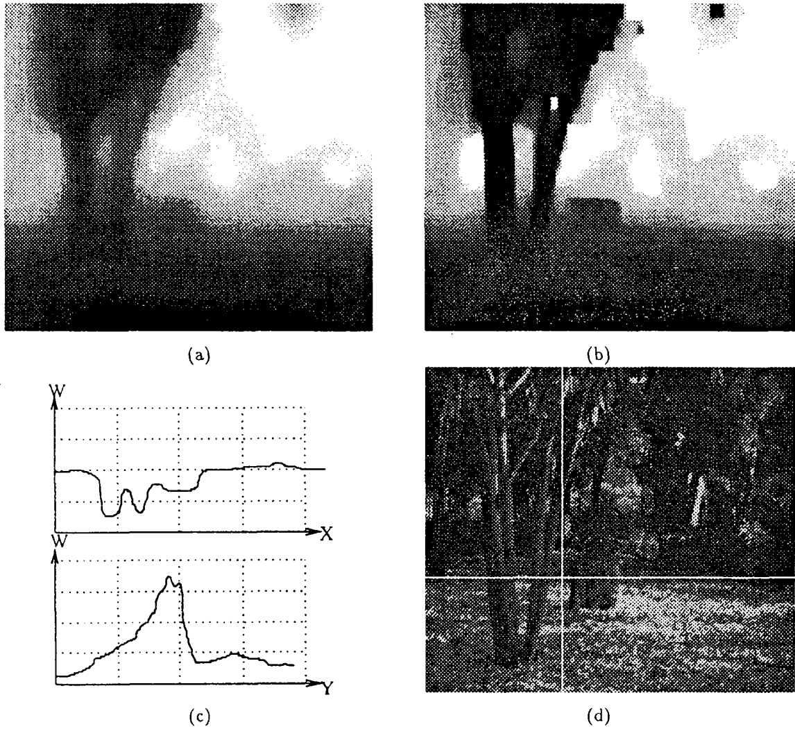
Figure 8: (a) Trees depth image computed by smoothing using the algorithm of section 3.1. (b) Depth image after four iterations of the iterative scheme of section 3.2. (c) Depth values along the horizontal and vertical lines plotted in (d). We have stretched the depth images to enhance the contrast so that the furthest areas appear completely white. Note that the trunks and the stump clearly stand out.
