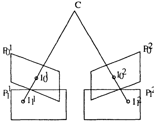
Figure B.2: Rectification of two images: the two original images I_0^1 and I_0^2 are rectified into I_1^1 and I_1^2 by reprojecting them to the same image plane P_1^1 = P_1^2 .
