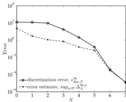
Figure 2. Convergence of the WEAKGREEDY N algorithm.
