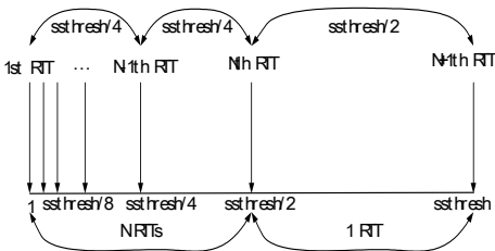
Fig. 3. Window change of slow start of TCP
