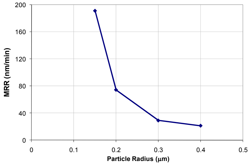
Figure 14: PAML prediction of MRR with varied inputs for abrasive particle radius
